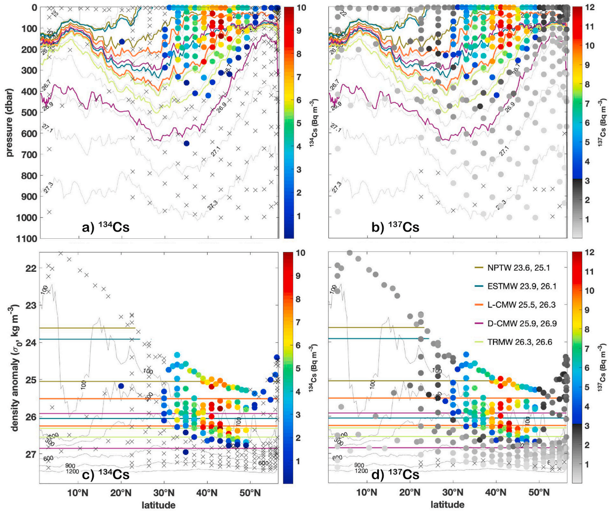
Fig. 3. a) ^{134}\text{Cs} along 152°W in latitude-pressure space. Colors indicate magnitude of activity decay corrected to April 6, 2011. Color bar is saturated at 10 Bq m -3 . Gray x symbols are values below detection limit; gray lines are potential density anomaly relative to 0 dbar; colored lines are boundaries for each Table 1 water mass according to the legend in (d); b) Same as (a) for ^{137}\text{Cs} . Color bar saturated at 12 Bq m -3 ; c) same as (a) in latitude- \sigma_t space with gray curves representing pressure contours; d) Same as (c) for ^{137}\text{Cs} . Note, ^{137}\text{Cs} gray scale below 3 Bq m -3 . This value has been chosen to facilitate comparison to the ^{134}\text{Cs} figure and to improve the representation of weaker signals. Although it is representative of the maximum remaining \text{Cs}_{\text{WT}} in the region, it should not be taken as a hard and fast estimate as \text{Cs}_{\text{WT}} has a latitudinal dependence (see Section 3.3). (For interpretation of the references to color in this figure legend, the reader is referred to the Web version of this article.)
