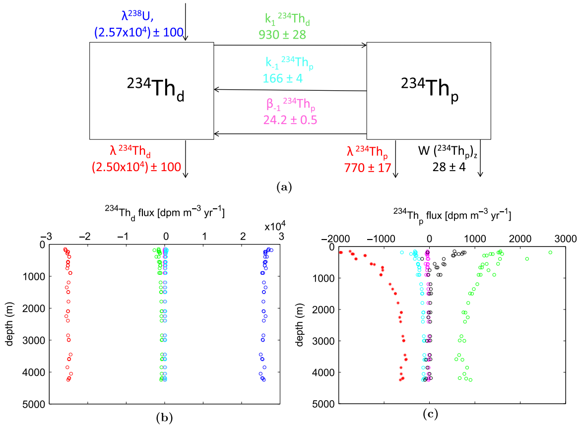
Fig. 15. Panel (a) shows the ^{234}\text{Th} budget at station GT11-22. The displayed values are vertical averages (125–4243 m) in \text{dpm m}^{-3} \text{yr}^{-1} . Panel (b) and (c) show the vertical distribution of the ^{234}\text{Th} fluxes. In all panels, red for radioactive decay, blue for radioactive production, green for adsorption, cyan for desorption, magenta for remineralization, and black for the sinking flux.
