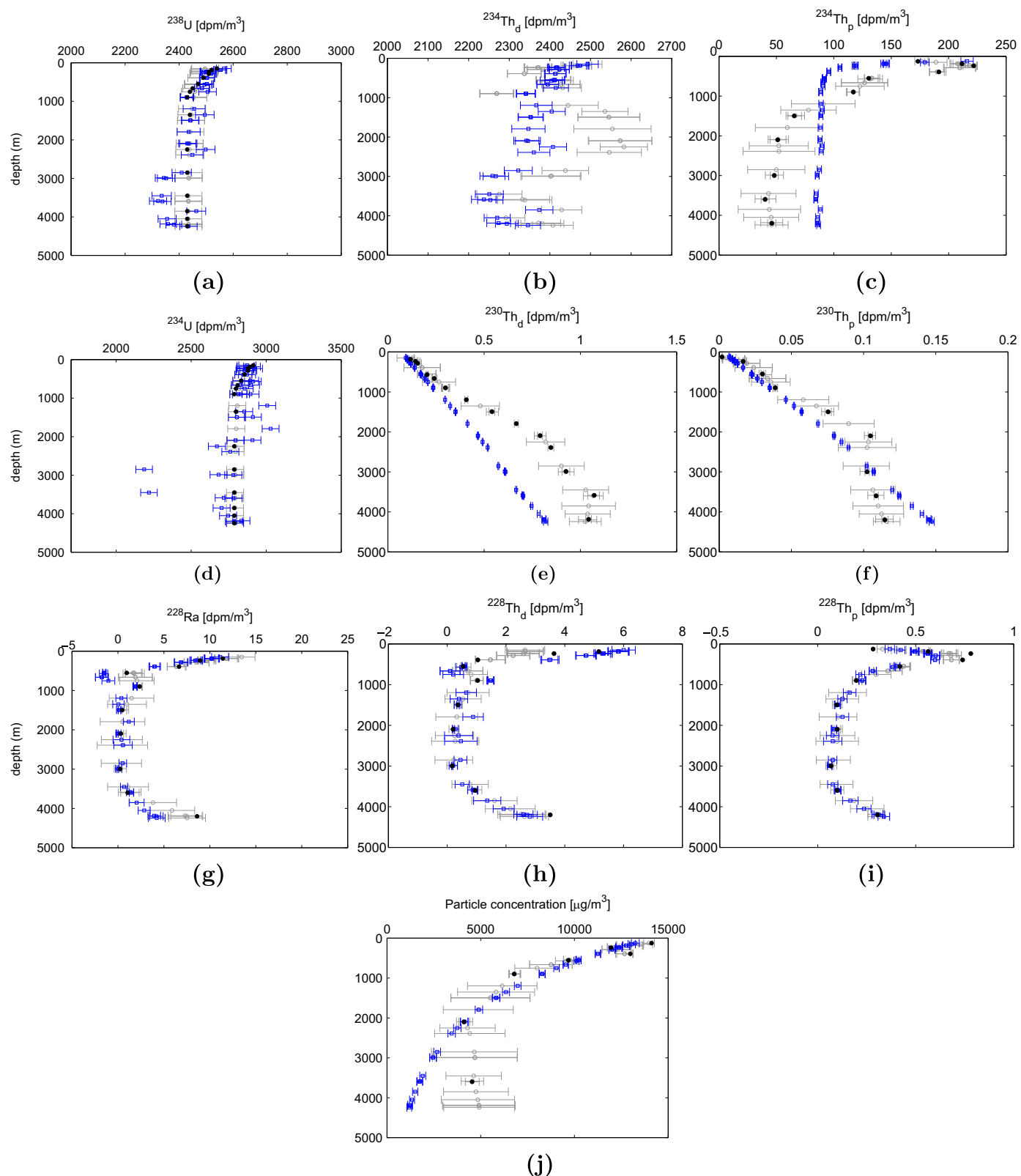
Fig. 7. Radiochemical activities and particle concentrations at station GT11-22. The black circles are the measured values, the open circles are the interpolated values, and the blue squares are the fitted values for model V1. Horizontal bars represent \pm 1 standard deviation.
