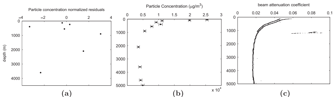
Fig. 19. Panel (a) portrays the normalized residuals for particle concentration (Eq. (11)). Panel (b) portrays the particle concentrations \pm 1 standard deviation from 125 m to 4989 m, the deepest depth at which small and large particles were sampled (data from Lam et al., 2015). Panel (c) shows the beam attenuation coefficient measured using a WET Labs 25 cm pathlength C-Star transmissometer (660 nm) (data from Anderson et al., 2013). The very large values between 1000 and 1500 m are real measurements.
