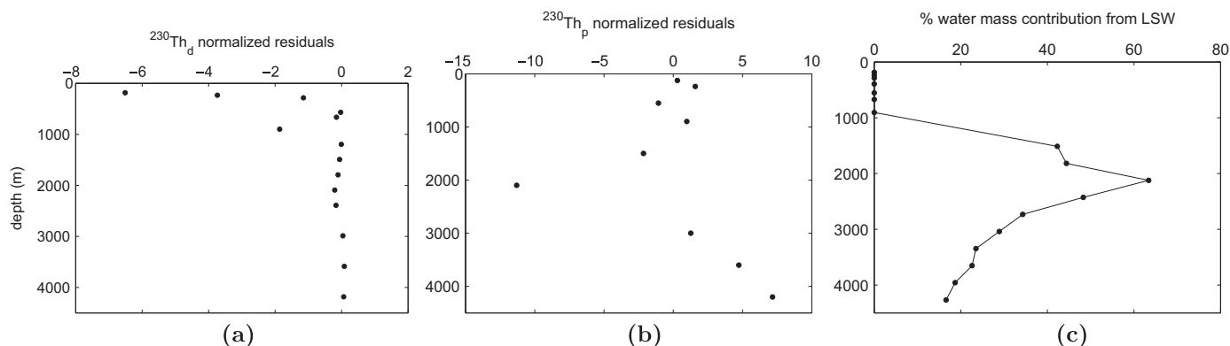
Fig. 18. Panel (a) and (b) show the normalized residuals (Eq. (11)) of ^{230}\text{Th}_d and ^{230}\text{Th}_p , respectively, for our reference solution (Section 3). Panel (c) shows the sum of the proportions of Upper Labrador Sea Water and Central Labrador Sea Water at station GT11-22 (estimates from Jenkins et al., 2015).
