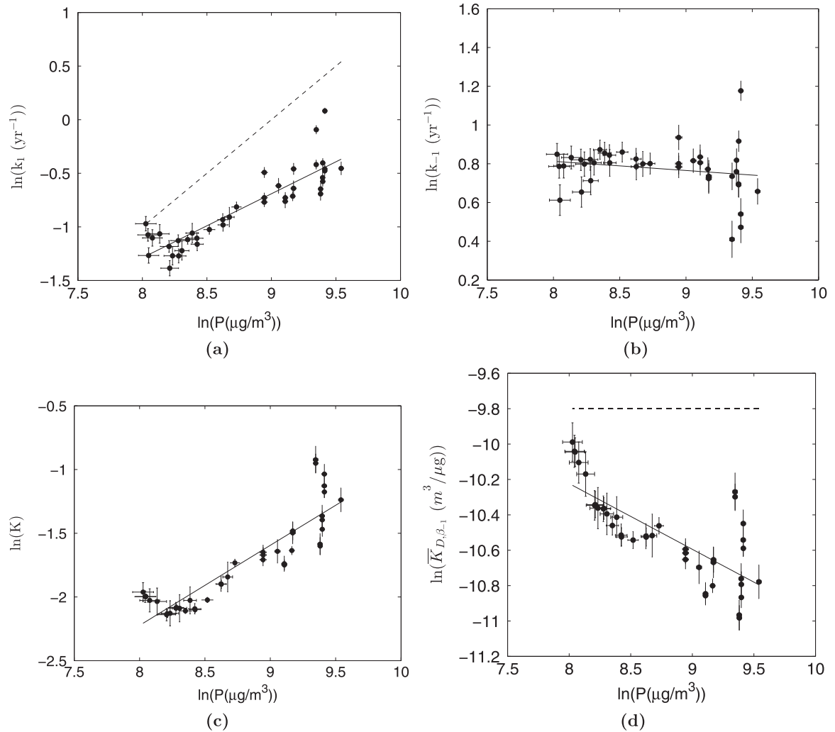
Fig. 14. Variation of k_1 (a), k_{-1} (b), K = k_1/(k_{-1} + \beta_{-1}) (c), and \bar{K}_{D,\beta-1} = K/P (d) with particle concentration, as inferred from inversion of station GT11-22 data. Horizontal and vertical bars show \pm 1 standard deviation. In each panel, the solid line is the ordinary least squares fit. The slopes of these lines are (a) 0.81 \pm 0.06 , (b) 0.06 \pm 0.03 (c) 0.73 \pm 0.06 , and (d) -0.28 \pm 0.06 . In panels (a) and (d), the dashed line represents the slope expected in the absence of a particle concentration effect (the slope of this dashed line is 1 in panel a, and 0 in panel d).
