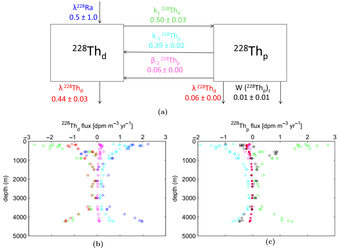
Fig. 16. Same as Fig. 15, but for ^{228}\text{Th} .
