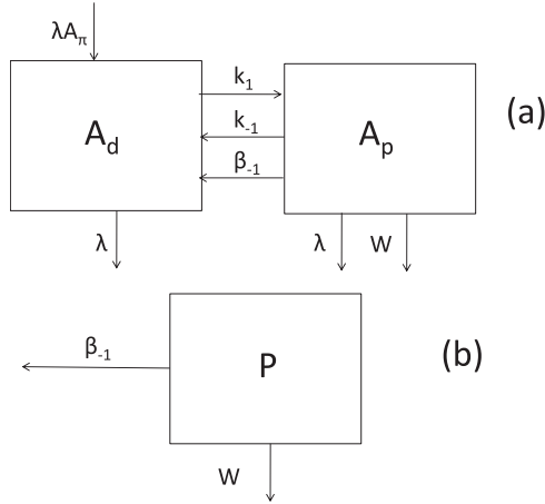
Fig. 6. Schematic diagram of the single-particle class model of Th cycling (a) and particle cycling (b). 'A' and 'P' represent, respectively, the Th isotope activity and the particle concentration in the dissolved fraction ('d') or the particulate fraction ('p'). A π is the activity of the parent isotope. The other symbols represent the rate parameters of solid-solution exchange (k 1 for adsorption, k -1 for desorption) and particle processes (β -1 for remineralization, and w for particle sinking). λ is the radioactive decay constant.
