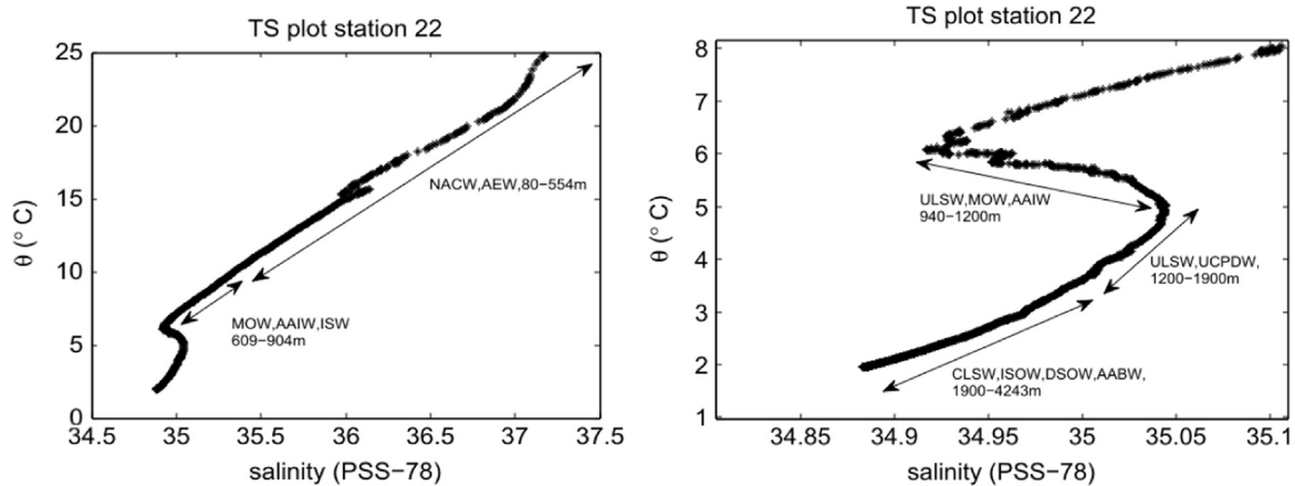
Fig. 2. Plot of potential temperature vs. salinity for station GT11-22. Arrows indicate the estimated range of water masses, with labels and the depth ranges. The left panel shows the \theta - S plot from the surface to a depth of 904 m. The right panel shows the \theta - S plot below 8 °C. Data from Jenkins et al. (2015).
