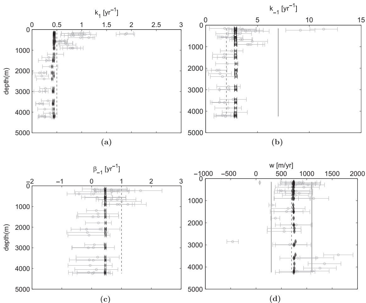
Fig. 12. Rate parameters of Th and particle cycling at station GT11-22 as inferred from the combination of data with model V2. The vertical dashed lines are the prior estimates, and the posterior estimates for \gamma=0.01 and \gamma=100 are represented by open grey circles and black squares, respectively. Horizontal bars are \pm 1 standard deviation. The solid lines show the range [value \pm one standard deviation] for the prior estimates.
