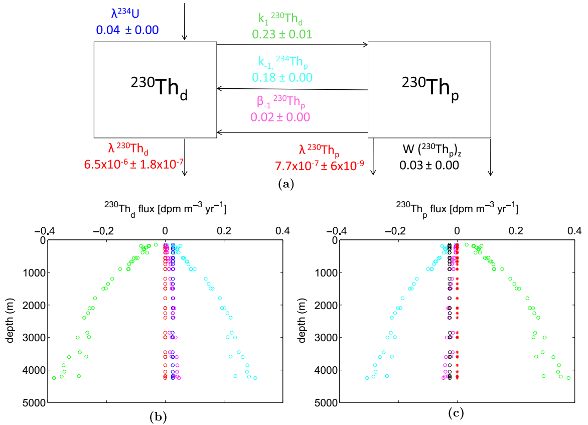
Fig. 17. Same as Fig. 15, but for ^{230}\text{Th} .
