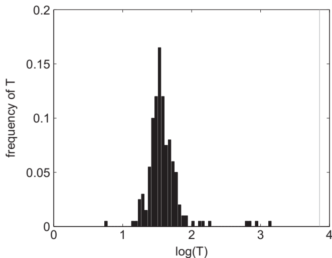
Fig. 9. Histogram of the frequency of the test statistic T obtained from the bootstrap. The grey line shows the value of T obtained from our reference solution (Section 3). The abscissa is the base-10 logarithm of the test statistic. Note that two negative values of T were found (−67 and −905), which are not shown in the figure.
