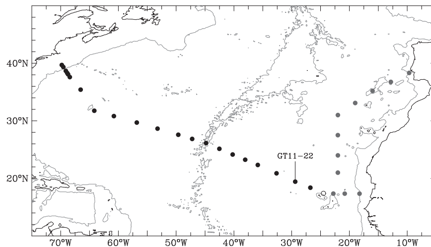
Fig. 1. Stations occupied by the R/V Knorr during the GEOTRACES North Atlantic section. The latitude and longitude of the stations are from http://data.bco-dmo.org/jg/dir/BCO/GEOTRACES/NorthAtlanticTransect/ . The grey dots show the stations occupied during the first leg (October 2010) and the black dots show the stations occupied during the second leg (November 2011). The open circle is both station 12 of the first leg and station 24 of the second leg. The data analyzed in this paper originate from station GT11-22, northwest of Cape Verde. The solid lines show the coastline (dark) and the 3000-m isobath (light) (bathymetric data are from http://www.ngdc.noaa.gov/mgg/global/ ).
