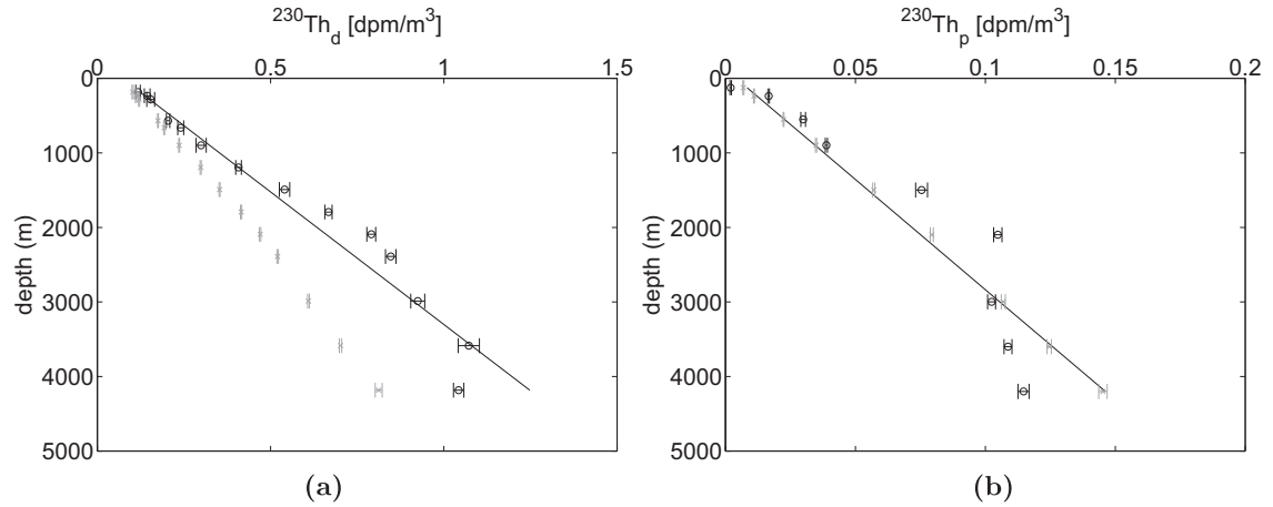
Fig. 11. The left panel shows the ^{230}\text{Th}_d measurements at station GT11-22 (open circles), the posterior estimates of ^{230}\text{Th}_d from the fit of model V1 (grey crosses) to the entire data set ( ^{234}\text{Th} , ^{238}\text{U} , ^{228}\text{Th} , ^{230}\text{Th} , ^{234}\text{Th} , ^{238}\text{U} ), and the line from fit of model V1 to only dissolved ^{230}\text{Th} data (derived from weighted least squares regression of ^{230}\text{Th}_d with depth). Horizontal bars are \pm 1 standard deviation. The right panel is the same as the left panel, but for ^{230}\text{Th}_p .
