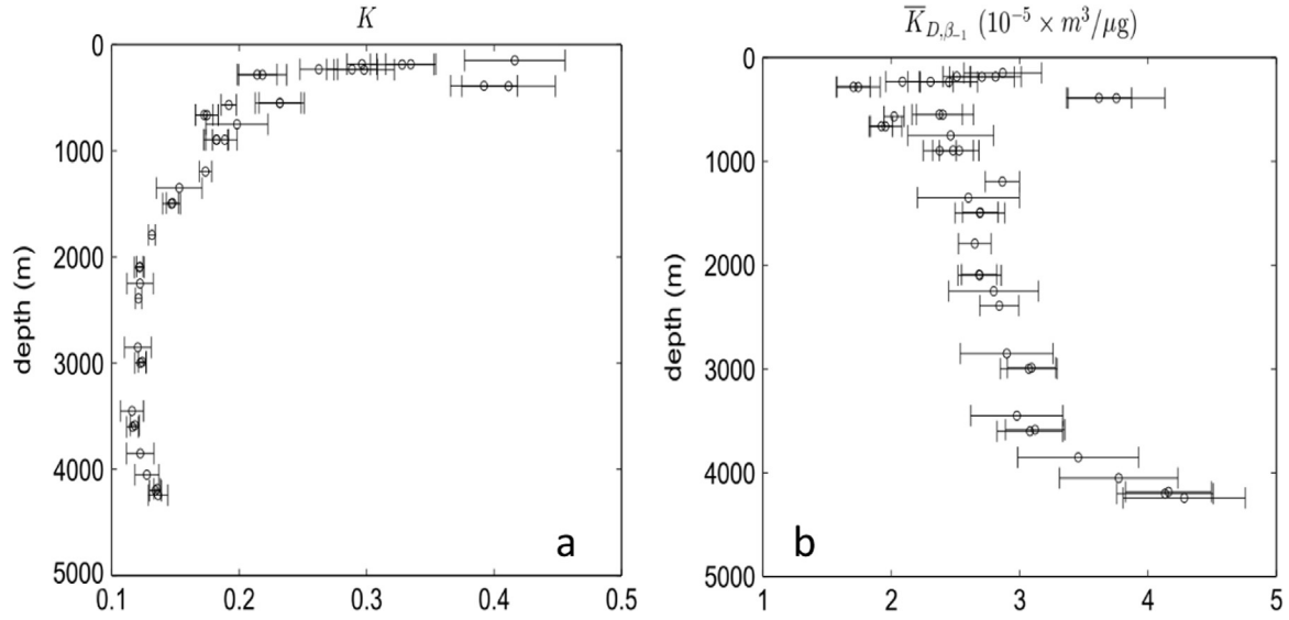
Fig. 13. Profiles of K = k_1/(k_{-1} + \beta_{-1}) (a) and \bar{K}_{D,\beta-1} = K/P (b) at station GT11-22, as inferred from the combination of data with model V2. The horizontal bars show the errors (one standard deviation) derived from propagating the posterior errors of k_1 , k_{-1} , \beta_{-1} (and P for \bar{K}_{D,\beta-1} ), with due regard for the error covariances.
