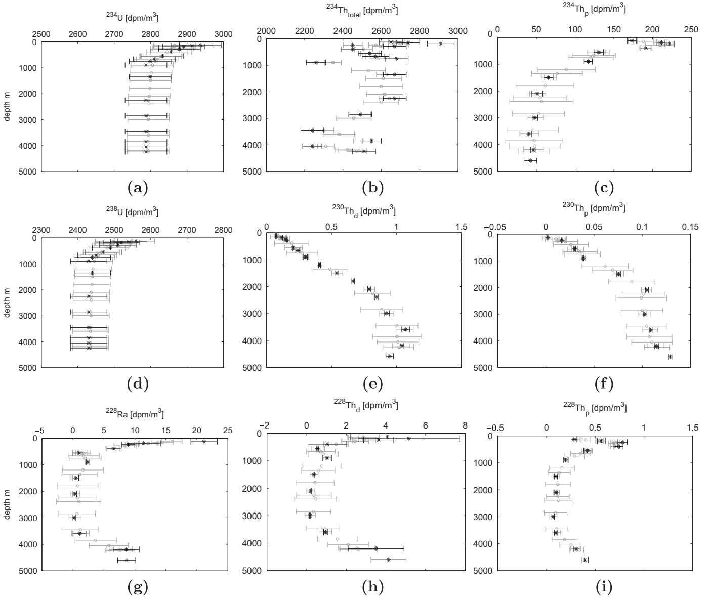
Fig. 5. Profiles of Th isotope activities and their parent activities at station GT11-22. The black asterisks are the measured values. The open circles are the interpolated values obtained with \sigma_M^2 = 0.5\sigma^2 , l_z = 1000 m. Horizontal bars show \pm 1 standard deviation.
