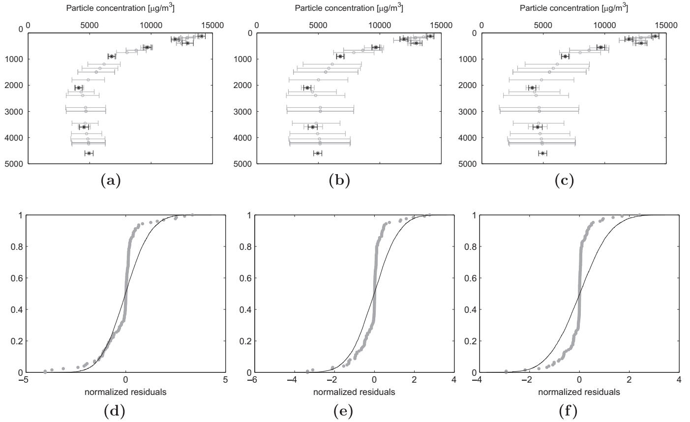
Fig. 3. Top row (a–c): Measured (black asterisks) and interpolated (open circles) values of particle concentration ( P ) at station GT11-22 for three different field property variances: \sigma_M^2 = 0.25\sigma_d^2 (a), \sigma_M^2 = 0.5\sigma_d^2 (b), and \sigma_M^2 = \sigma_d^2 (c), where \sigma_d^2 is the variance of P measurements at station GT11-22. A length scale of l_z = 1000 m is used for each panel. Horizontal bars show \pm 1 standard deviation. Measured particle concentrations are from Lam et al. (2015). The deepest measured value used in the interpolation of particle concentration is at 4600 m. Bottom row (d–f): Distribution function (DF) of the interpolation residuals normalized to measurement errors for all GT11-22 data used in this study. A normalized residual is defined as (\hat{x}_i - x_{d,i})/\sigma_{d,i} , where \hat{x}_i is the interpolated value at measurement depth level i , x_{d,i} is the measured value at this level, and \sigma_{d,i} is the error in the measurement at this level. For the three values of \sigma_M^2 , the difference |\hat{x}_i - x_{d,i}| is less than 2\sigma_{d,i} for more than 95% of the data, which suggests an overfit (the solid line shows the normal DF).
