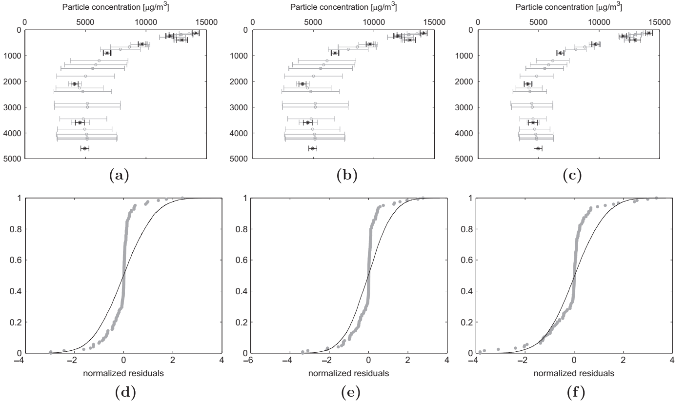
Fig. 4. Same as Fig. 3, but for three different vertical correlation scales: l_z = 500 m (a), l_z = 1000 m (b), and l_z = 2000 m (c). A field property variance of \sigma_M^2 = 0.5\sigma_d^2 is used for each panel. Measured particle concentrations are from Lam et al. (2015).
