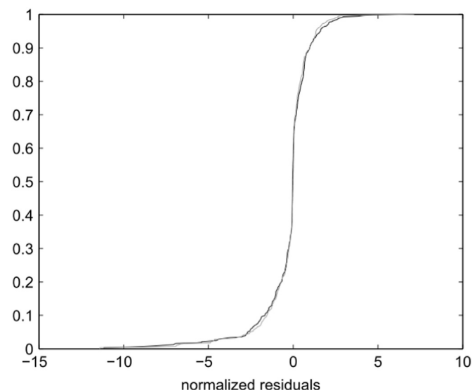
Fig. B1. Normalized residuals of the fit of model V2 to station GT11-22 data for the reference case (Section 3) (black), and for the case where the prior ^{228,234}\text{Th}_p values are set to 20% less than their measured values (grey).
