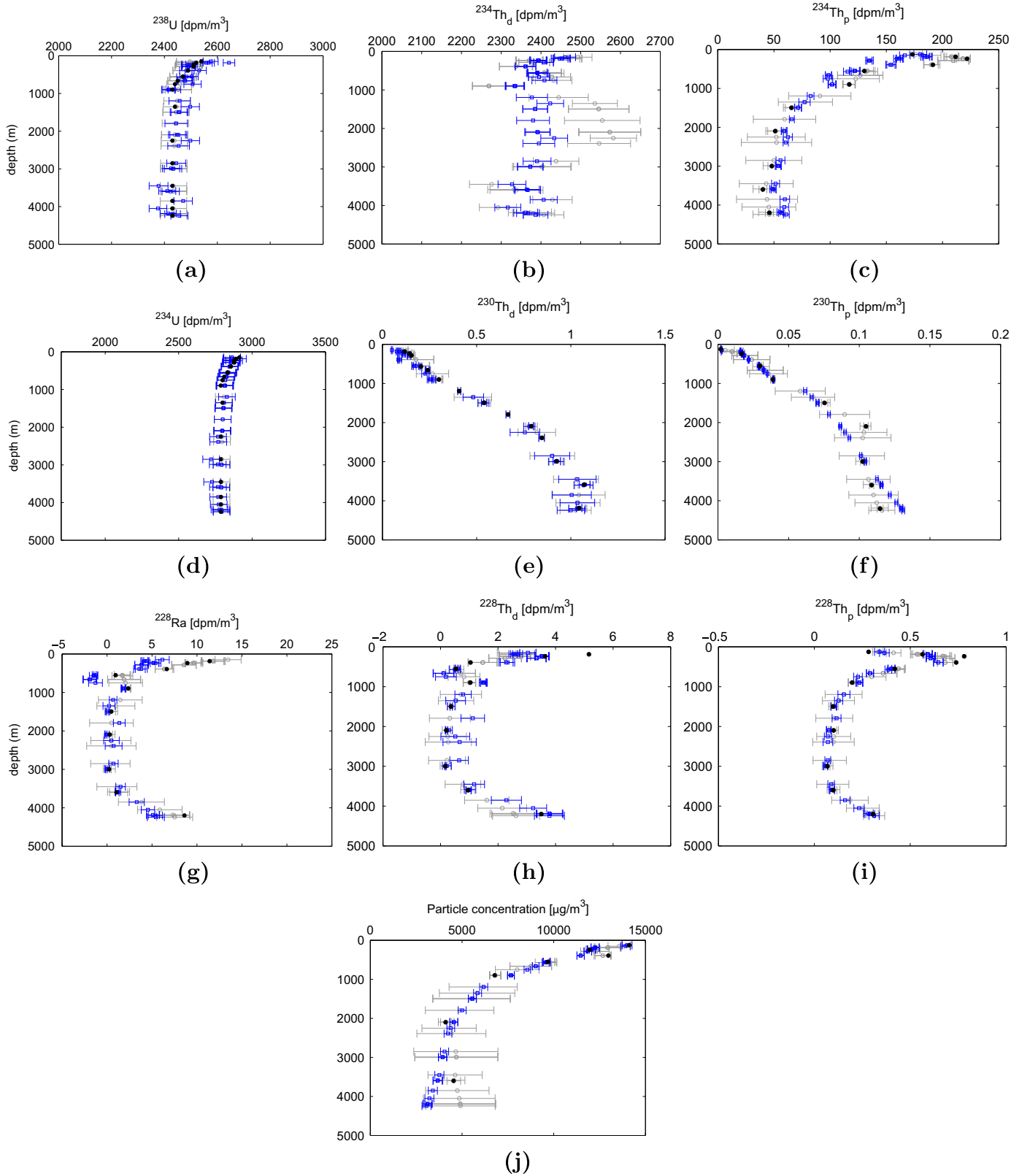
Fig. 8. Same as Fig. 7, but for model V2.
