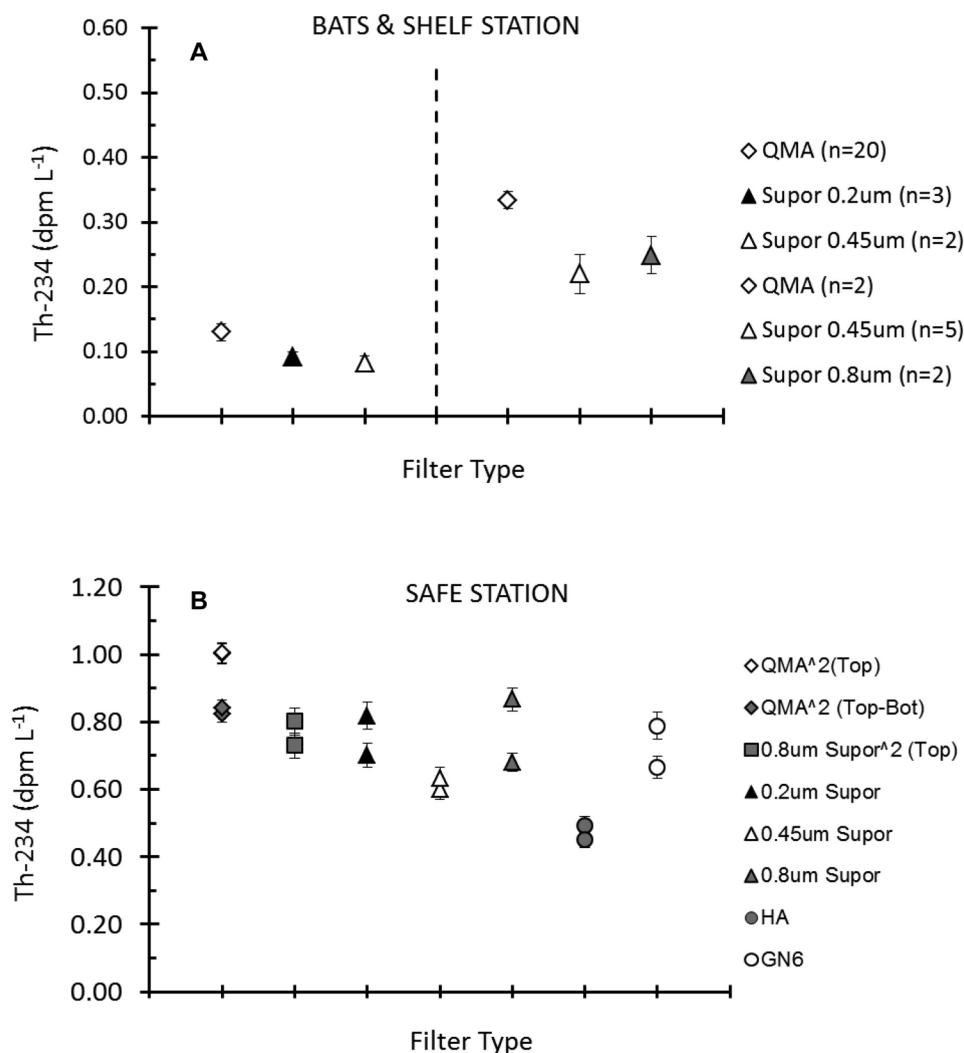
Fig. 6. Different filter types affecting ^{234}\text{Th} activity on small particles. Two subsamples from each filter type ( n = 2 ) is analyzed for SAFE station.
