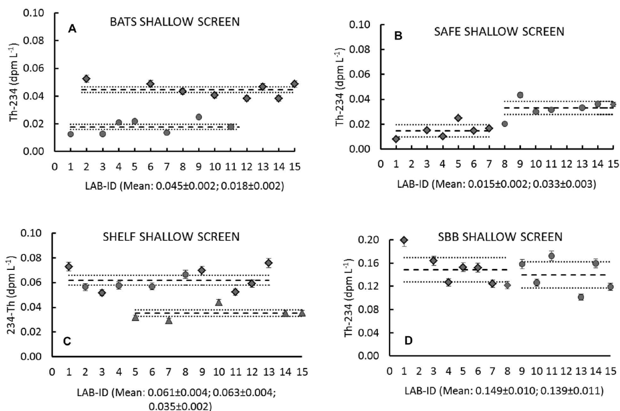
Fig. 5. Intercalibration results for large particles. Each symbol represents samples collected from a particular cast. The dashed line associated with each symbol represents the mean 234 Th activity for the cast. The dotted lines represent 95% confidence interval.
