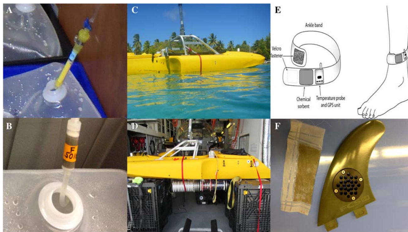
Fig. 1 Sampling methods. a AMP-PAN column; b KNiFC-PAN column; c JetYak; d Rad Clio on JetYak; e RadBand design; f Radband mesh bag & surf fin designed to hold RadBand
