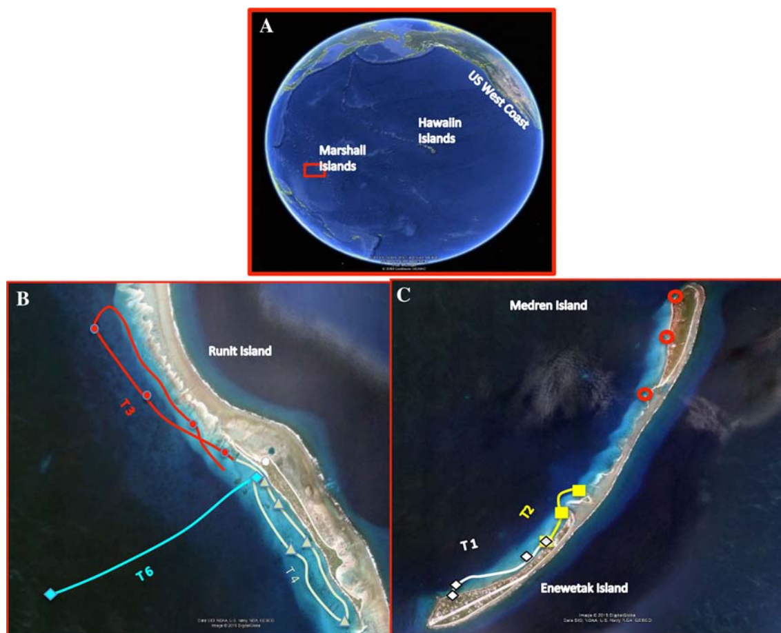
Fig. 2 Marshall Islands. a Red square represents Marshall Islands chain. b Runit Island with transects 3 (red), 4 (white), 6 (aqua) with co-located cubitainer samples and stationary sample 5 (aqua circle
